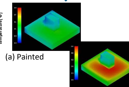
(b) no-painted Effect of reflective paint
