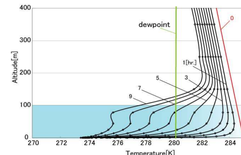
Atmospheric temperature (particle diameter increases)
