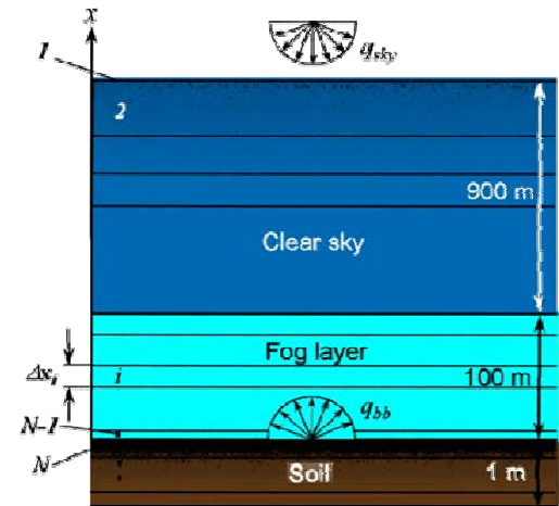
Plane parallel system for fog formation prediction
