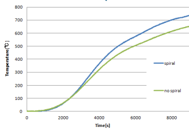
Transition of the furnace temperature
