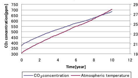
Global warming prediction
