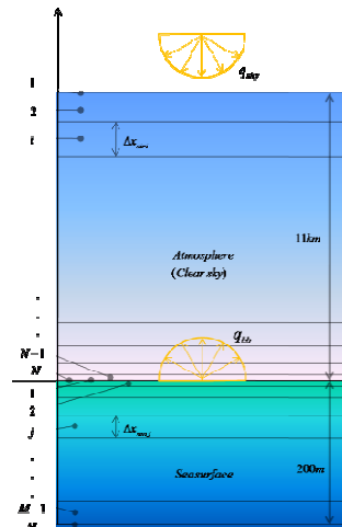
Plane parallel system for global warming prediction
